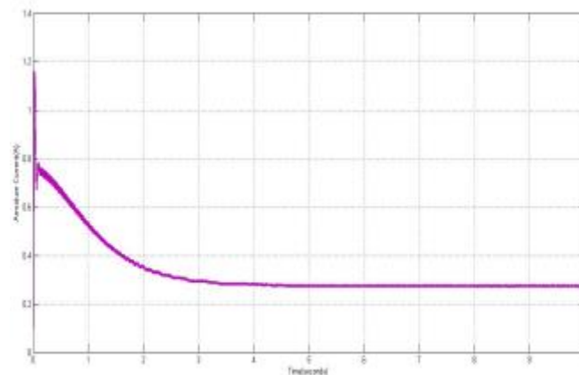
Fig.4: Armature Current
