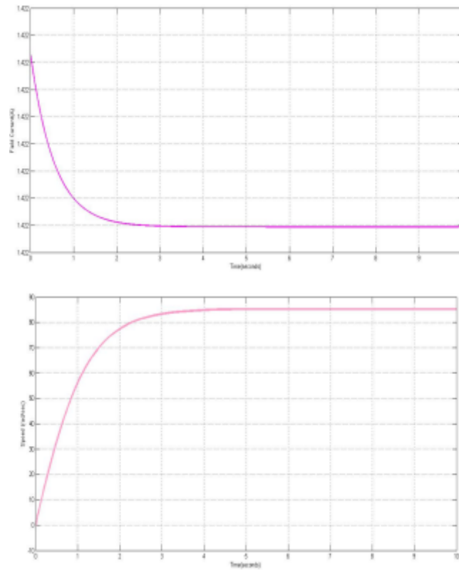
Fig.3: Speed of DC Motor
