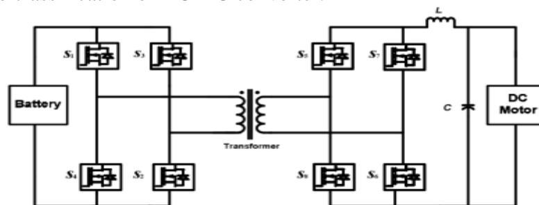
Fig.1: Isolated DC-DC Converter
